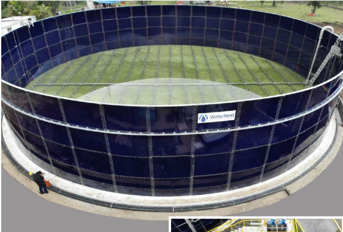
Diffuser Installation in circular Tank in Mexico for a plant for flow 2800 mcd
